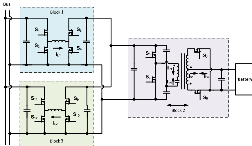
Figure 2. Topology of this new isolated bi-directional DC-DC converter
