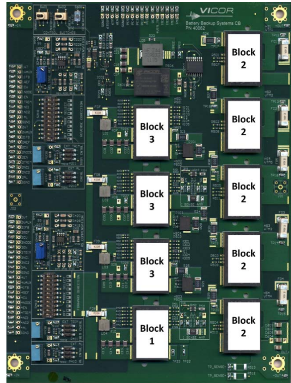
Figure 7. System implementation.
