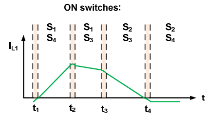
Figure 4. Block 1: current flowing through the inductor with ZVS intervals
