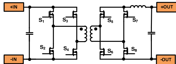
Figure 1. An existing isolated bi-directional DC-DC converter topology
