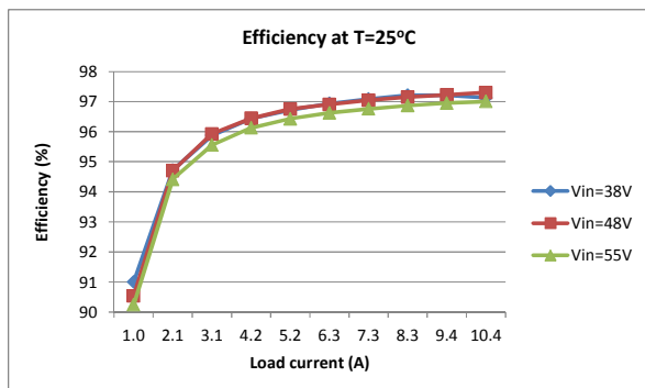
Figure 6. Experimental results of efficiency for a block 1 / block 3 module (500W, room temperature)
