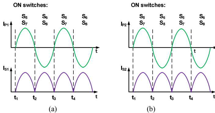
Figure 3. Block 2: Primary and secondary resonant current flows bi-directionally: (a) charging-battery direction; (b) supporting-bus direction
