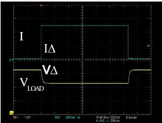
A battery simulator emulates the battery's voltage drop, \Delta V , due to its internal resistance when the load current changes near instantaneously by \Delta I .
