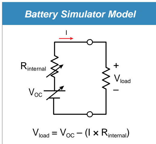
A battery simulator models the battery with a variable source and a variable internal resistance.
