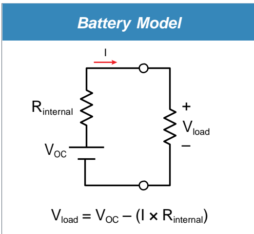
Simplified model of a battery: an ideal source with an internal resistance.
