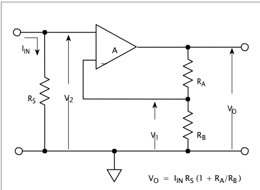
Shunt Ammeter
