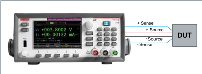
Series 2280S using rear output connector with remote sensing
